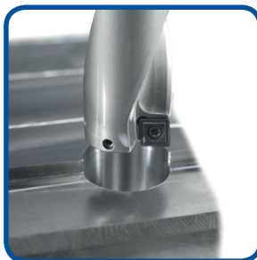
Katmanlı delme Rack drilling
